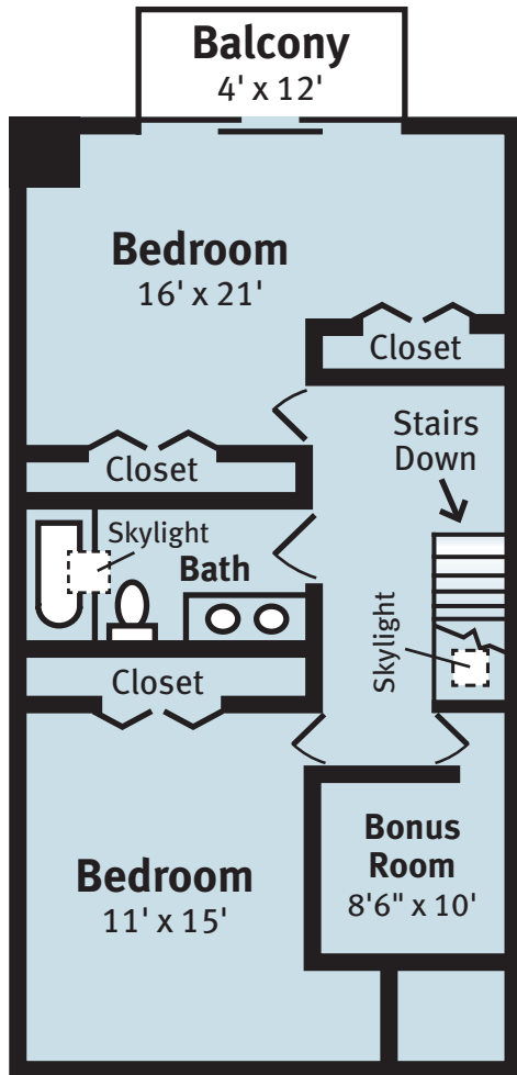
Upper Level
